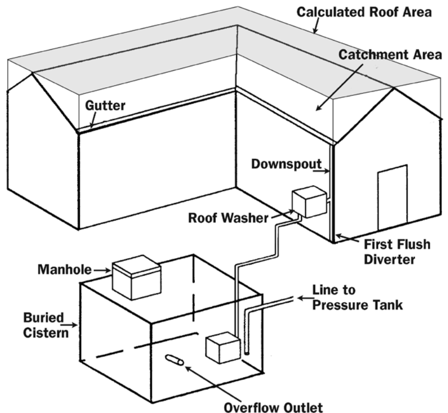
Figure 1. Basic rainwater harvesting system
