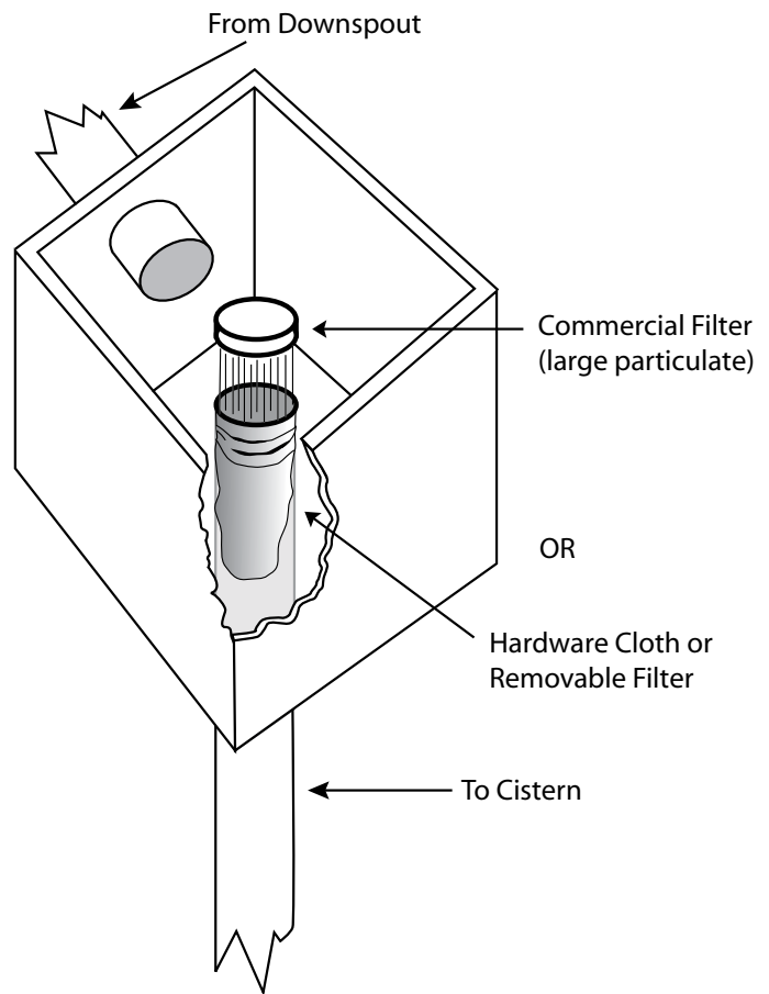
Figure 3. Basic roof washer design
