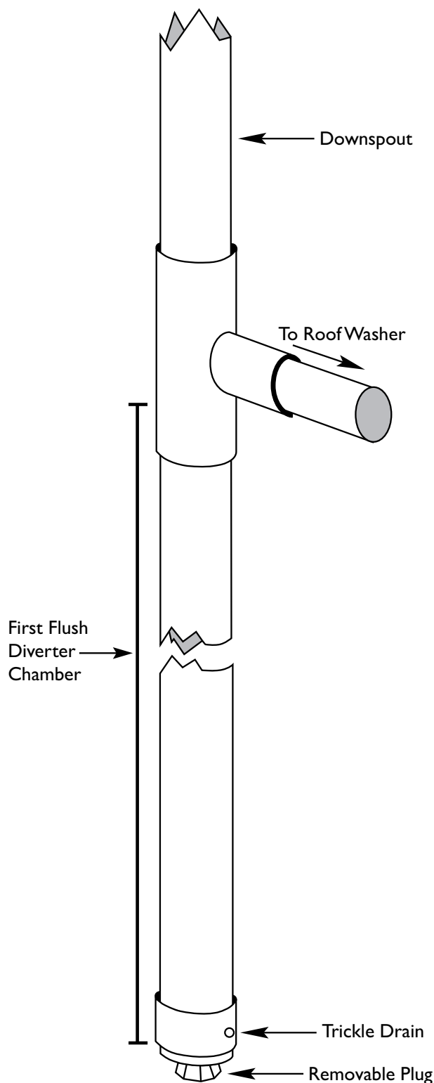
Figure 2. Basic first flush diverter design
