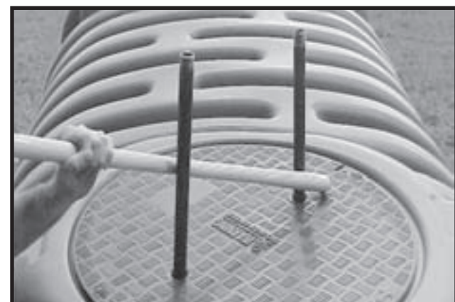
FIG.7 Remove Cover
