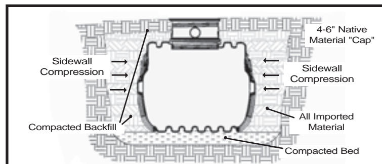
FIG.4 Backfilling
