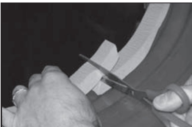
FIG.3 Trim Gasket
