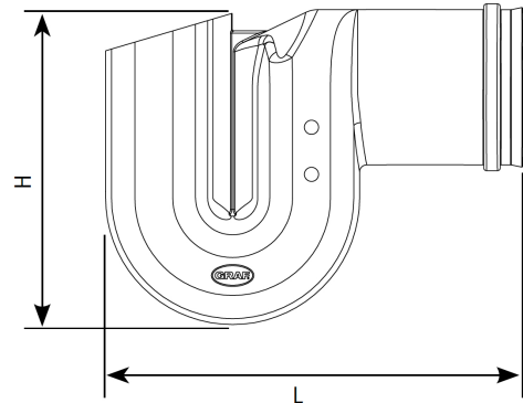
DN 200 (8") (with sleeve)
