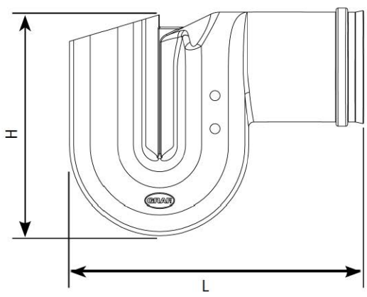
DN 300 (12") (with sleeve)
