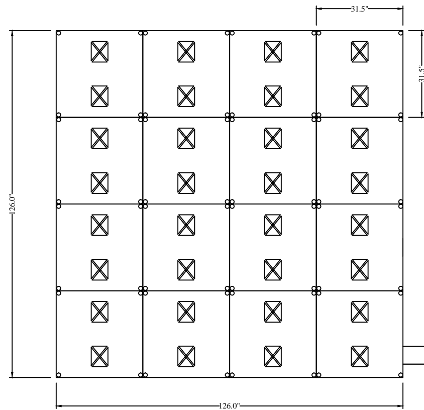
System Plan View
