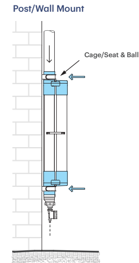
Figure 2 Delta Post/Wall - Inlet/Outlet Positions
