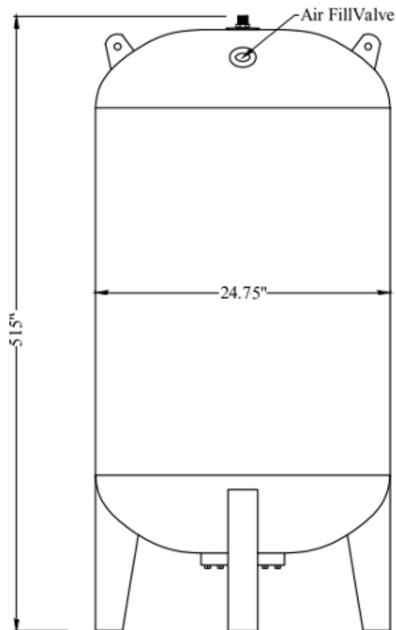
Side View
