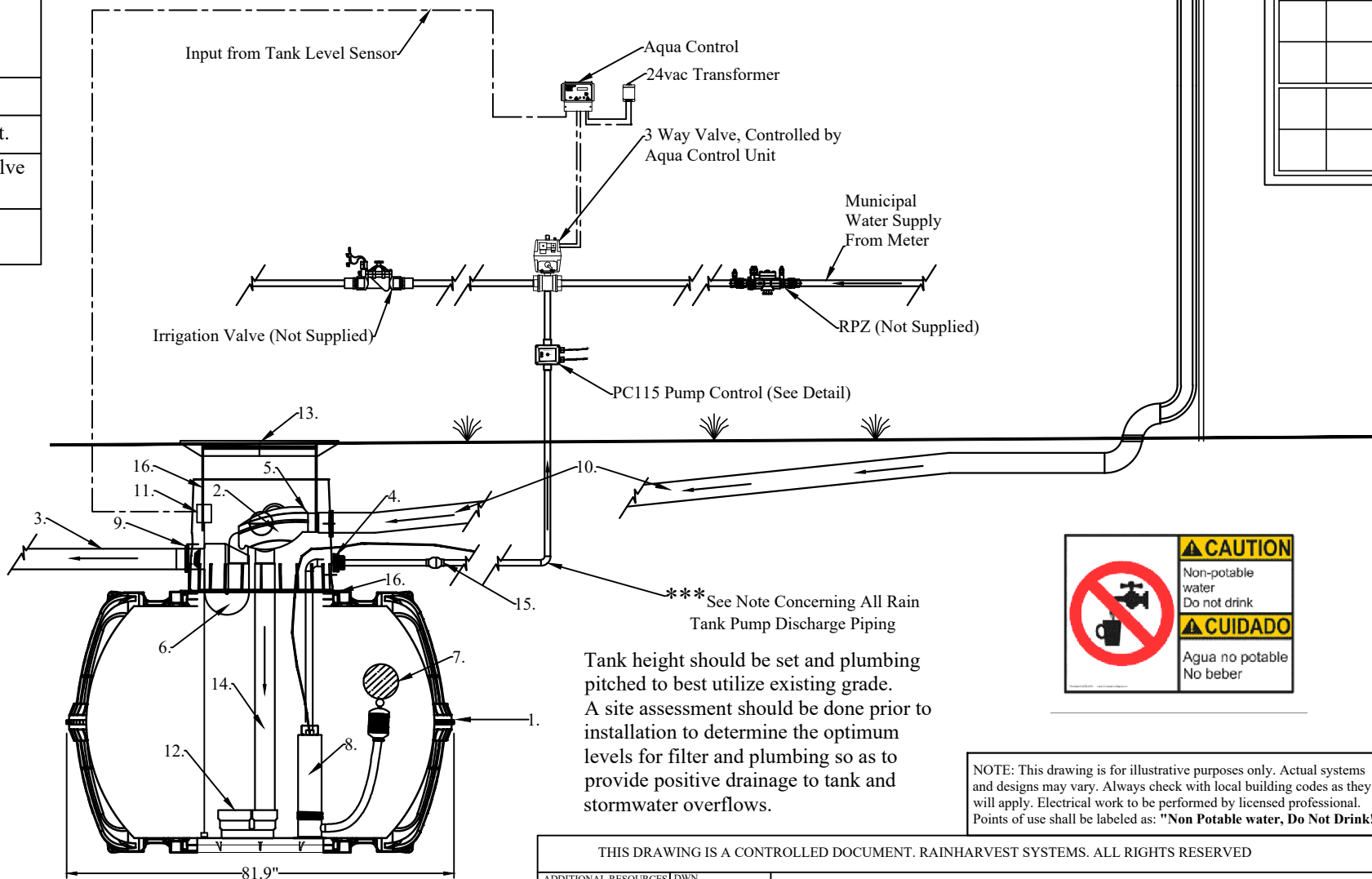
700 Gallon Carat Tank Cutaway Side View
