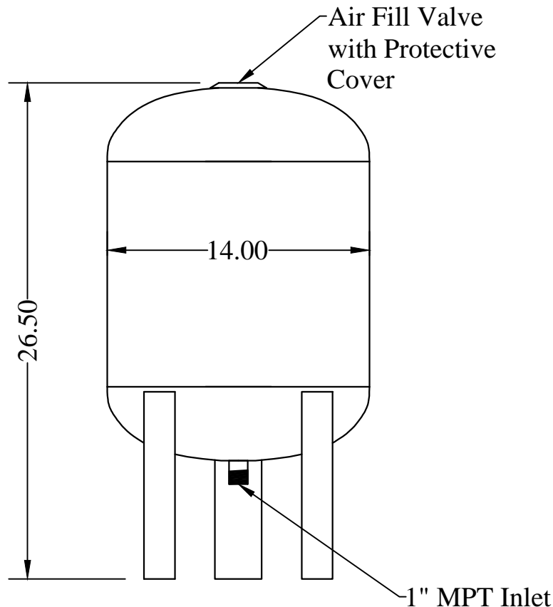
Side View
